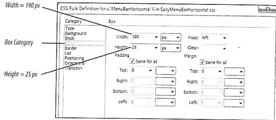
Figure 20 Add properties to the ul.MenuBarHorizontal li rule
